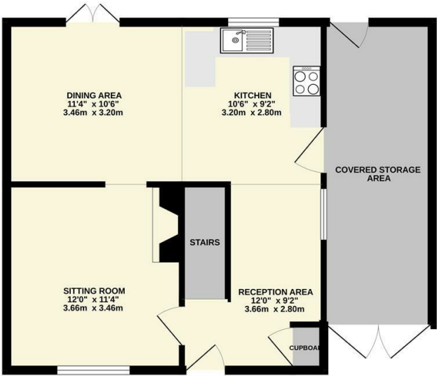
GROUND FLOOR 591 sq.ft. (54.9 sq.m.) approx.
